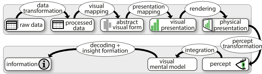
Fig. 26: Extended infovis pipeline that captures data physicalizations [70].
