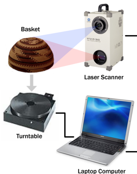
Fig. 2. A schematic representation of the scanning setup
