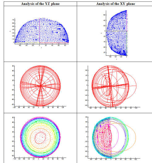
Fig. 8. Geometric analysis of a basket. Once transformed to the canonical orientation, the curvature of a basket can be obtained by taking slices along the x-y and y-z planes and fitting ellipses to the slices.
