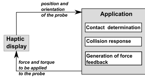
Figure 2. Haptic rendering pipeline
