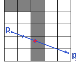
Figure 3. The ray from the previous position p_1 to the current one p_2 is cast with 1-voxel step until an obstacle is found or p_2 is reached
