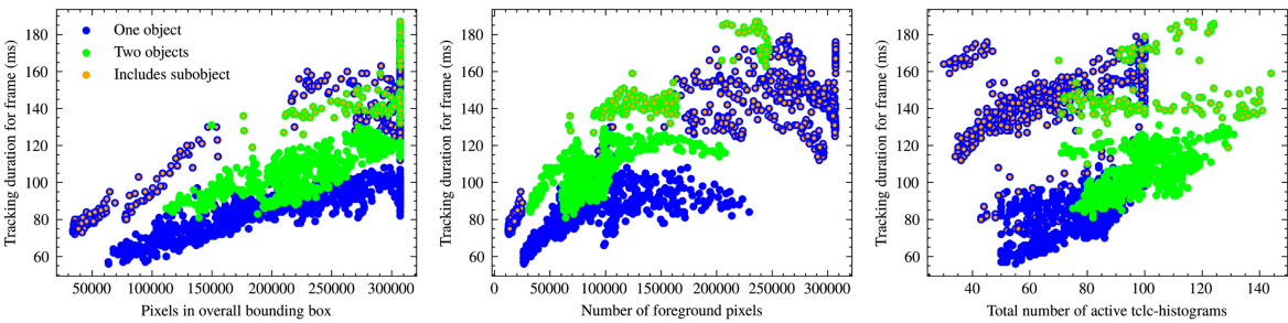
FIGURE 9. Scatter plots of sample tracking runtimes. Each dot represents the tracking runtime for a single frame of video. Here, “bounding box” denotes the single 2-D rectangle containing all objects’ silhouettes, and “number of foreground pixels” denotes the number of pixels the objects’ silhouettes occupy. “Active” tclc-histograms are ones that a frame’s calculations use. Since these metrics can vary slightly within a frame’s processing as the predicted pose incrementally updates, we recorded values at frames’ beginnings.
